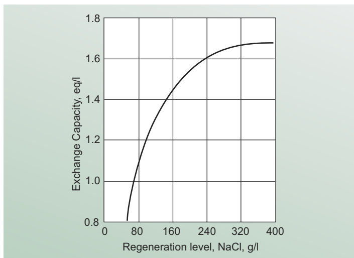
Fig. 1 Exchange capacity vs. regeneration level Sodium form C-800x10 Cation Resin
