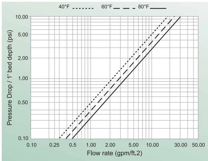
Fig. 1 Pressure Drop vs Flow Rate at various degrees Fahrenheit (F°)
